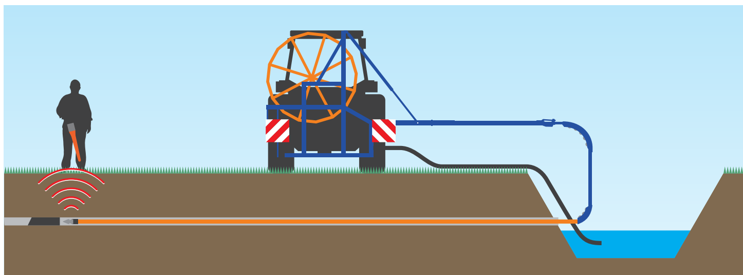
Easyloc Tx Signal Transmitter
